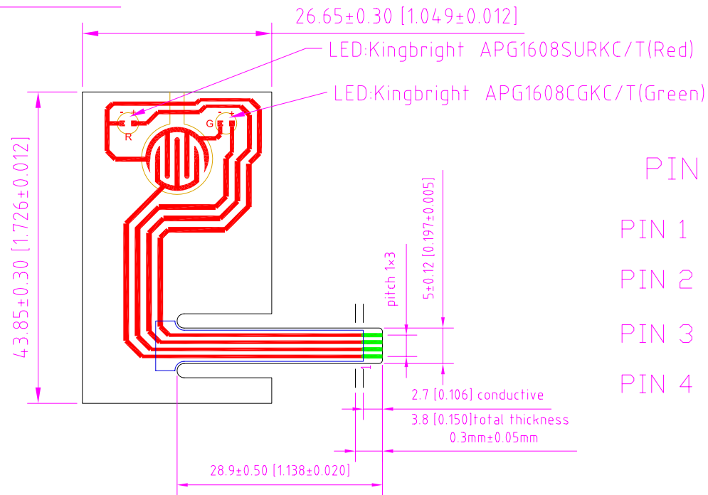
Lower circuit
